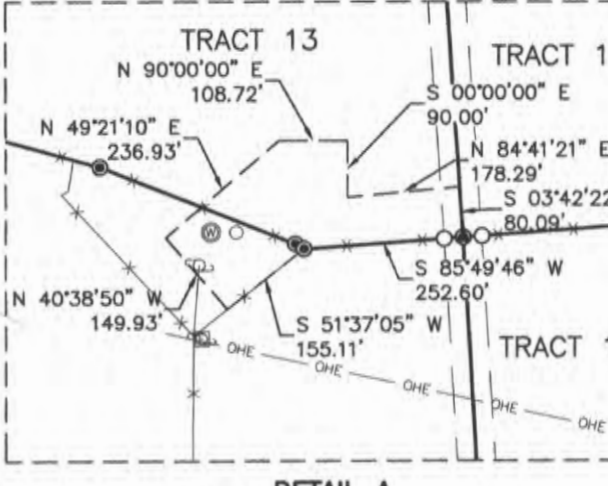
DETAIL A WATER WELL EASEMENT SCALE 1"=300'
